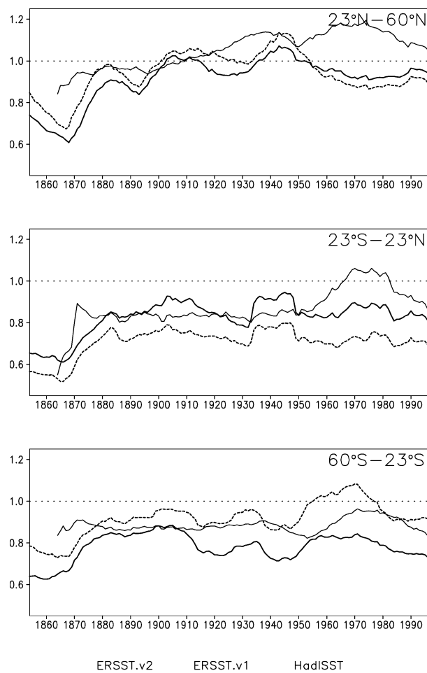
FIG. 7. Temporal standard deviation ratios, as in Fig. 2, except in the areas 23^{\circ} – 60^{\circ} N, 23^{\circ} S– 23^{\circ} N, and 60^{\circ} – 23^{\circ} S for ERSST.v2, ERSST.v1, and HadISST.
