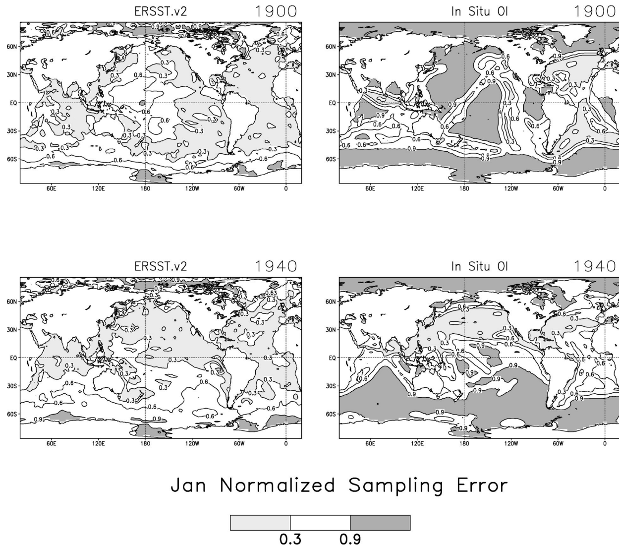
FIG. 9. For (left) ERSST.v2 and (right) the in situ OI, monthly normalized sampling standard error for January of 1900 and 1940. Values below 0.3 and above 0.9 are shaded.
