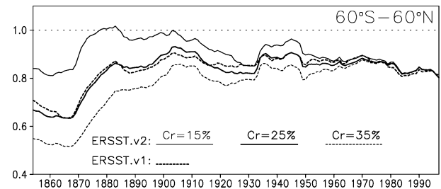
FIG. 2. Ratios of temporal standard deviations from 15-yr running periods to the 1982–97 NOAA OI standard deviation, averaged over 60^{\circ}\text{S} – 60^{\circ}\text{N} . The ERSST.v2 ratios with different critical values are shown. For comparison the ERSST.v1 ratio is also shown.
