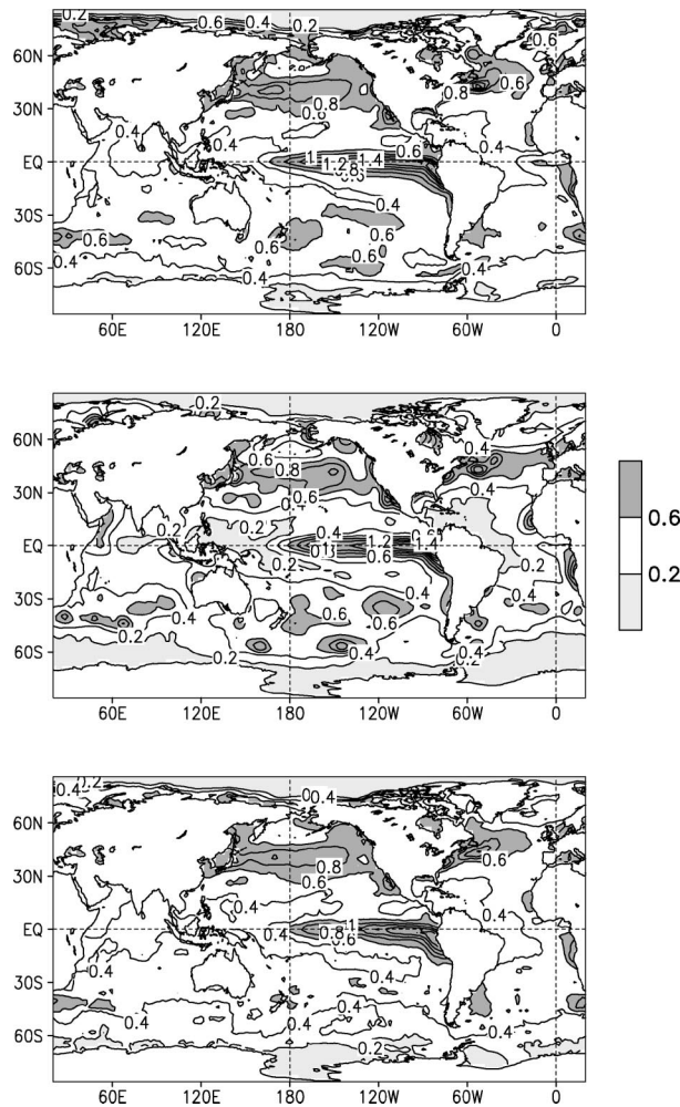
FIG. 1. Standard deviation of monthly SST anomalies over the 1982–97 period from the (top) NOAA OI, (middle) ERSST.v1, and (bottom) in situ OI. Values less than 0.2^{\circ} and more than 0.6^{\circ}\text{C} are shaded.
