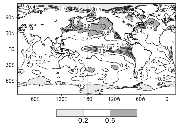
FIG. 3. Standard deviation of monthly SST anomalies over the 1982–97 period from the ERSST.v2 analysis using 3 months of data centered on the analysis month. Values less than 0.2^{\circ} and more than 0.6^{\circ}\text{C} are shaded.
