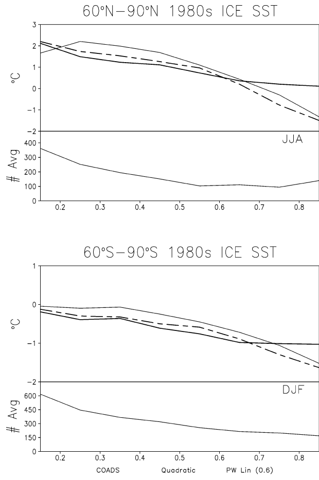
FIG. 4. Average 60° latitude to the pole SST from COADS and ERSST.v2 using the quadratic method and a piecewise linear method. Temperatures are shown for the warm season in each hemisphere, and are only averaged where collocated with a COADS observation. Also shown is the number of seasonal observations averaged for each SST. The horizontal axis is sea ice concentration in tenths.
