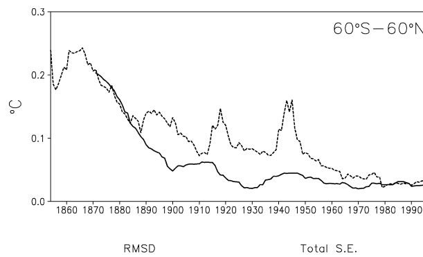
FIG. 8. For the ERSST.v2 annual and 60^{\circ} S– 60^{\circ} N average, the total standard error and the rmsd from the average HadISST analysis.
