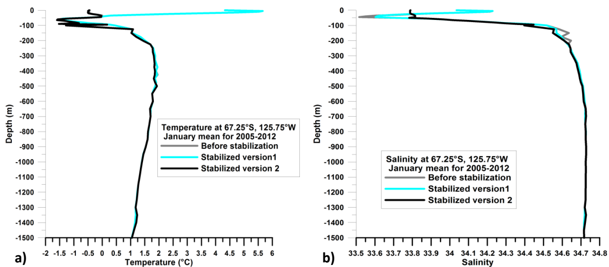
Figure 4: Vertical profiles at grid point 67.25°S, 125.75°W (location within warm feature in Figure 3a) for a) temperature and b) salinity. Stabilization in version 1 is set up to make the minimal adjustment to achieve stability, in this case resulting in anomalously high temperatures at the surface. Stabilization in version 2 adjusts only salinity.
