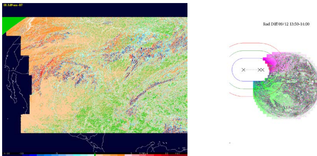
Figure 16: Example of IR stray light at night. The left panel shows the T_B (3.9 \mu\text{m} ) change in five minutes, the closer to the Sun, the larger the T_B change. Note also that the colder the scene, the larger the T_B change, even for scene fairly far away from the Sun. The right panel illustrates the size of Restricted Zone (blue) and the Zone of Reduced Data Quality (ZRDQ, red).
