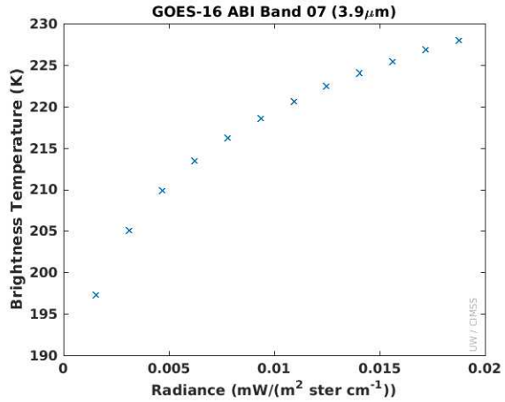
Figure 17: Planck relationship between brightness temperature and radiance for Band 7 (3.90 μm), displayed over the full dynamic range of the ABI band (left) and zoomed in to show the large discrete steps in brightness temperature at the cold (low radiance) end of the ABI L1b radiance range. A small amount of noise in the radiance values can be exaggerated into very large brightness temperature noise (plots courtesy UW/CIMSS Satellite Blog linked in the text).
