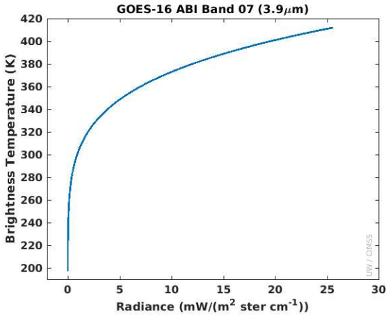
Figure 17: Planck relationship between brightness temperature and radiance for Band 7 (3.90 μm), displayed over the full dynamic range of the ABI band (left) and zoomed in to show the large discrete steps in brightness temperature at the cold (low radiance) end of the ABI L1b radiance range. A small amount of noise in the radiance values can be exaggerated into very large brightness temperature noise (plots courtesy UW/CIMSS Satellite Blog linked in the text).
